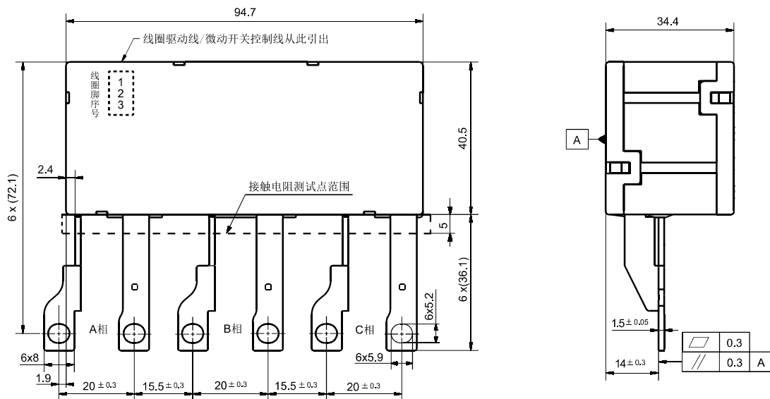
HFE45-3SH/3SD(双触点)
